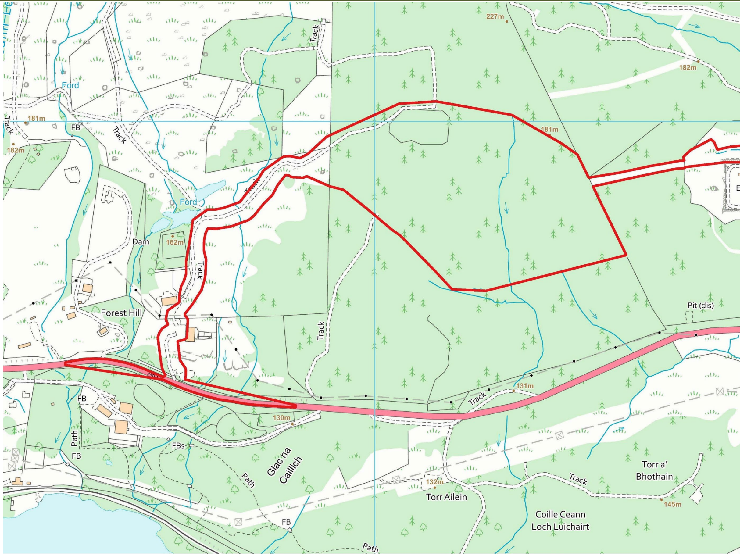
Figure 4.1: Forestry
