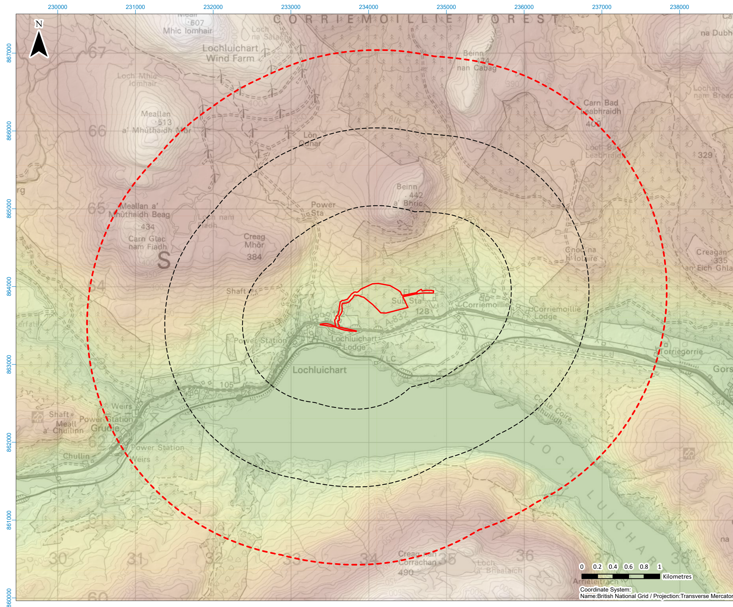
Figure 5.2: Topography
